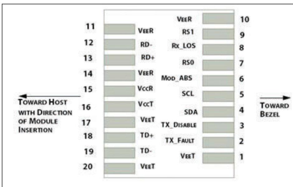
Figure 2: Module Interface to Host
