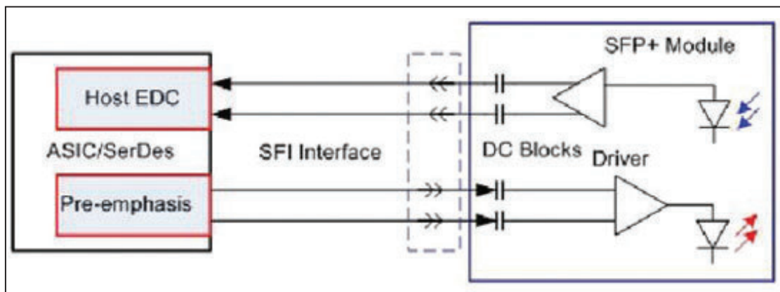
Figure1: Application in System
